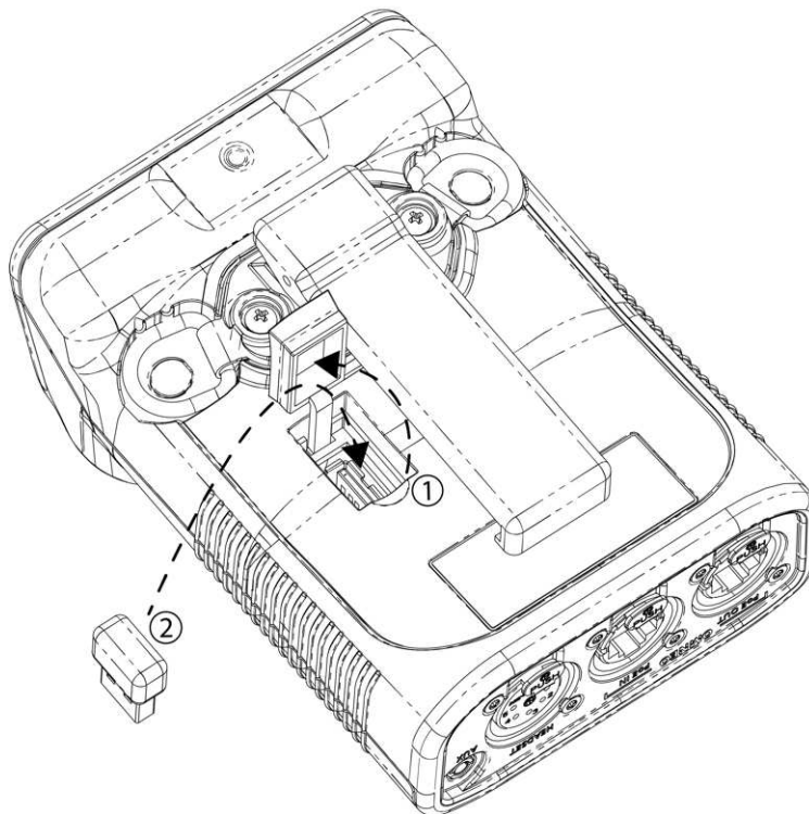
Figure 5.1: DBP USB dongle installation
